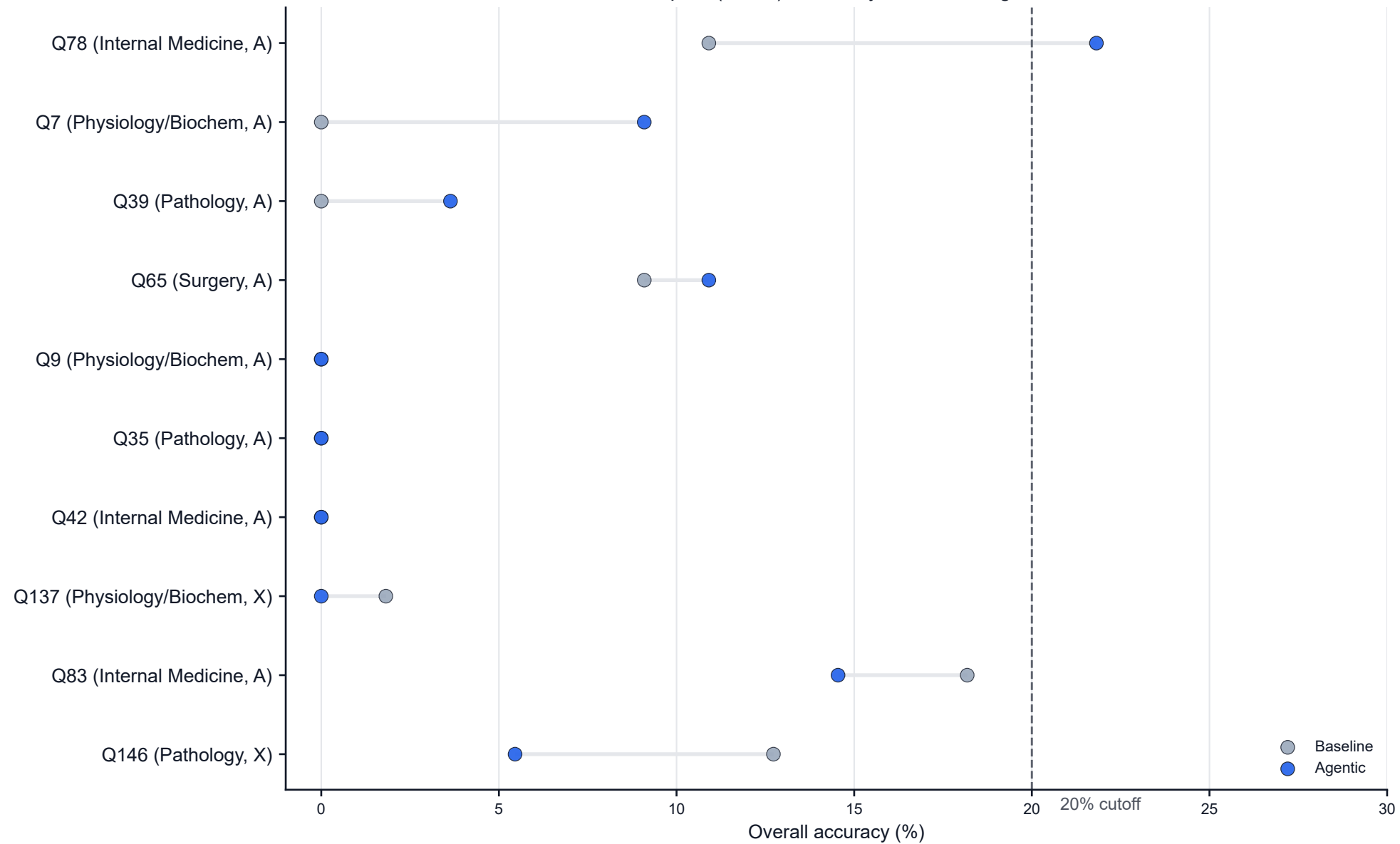
Baseline cold spots (<20%): accuracy shift under agentic workflow
